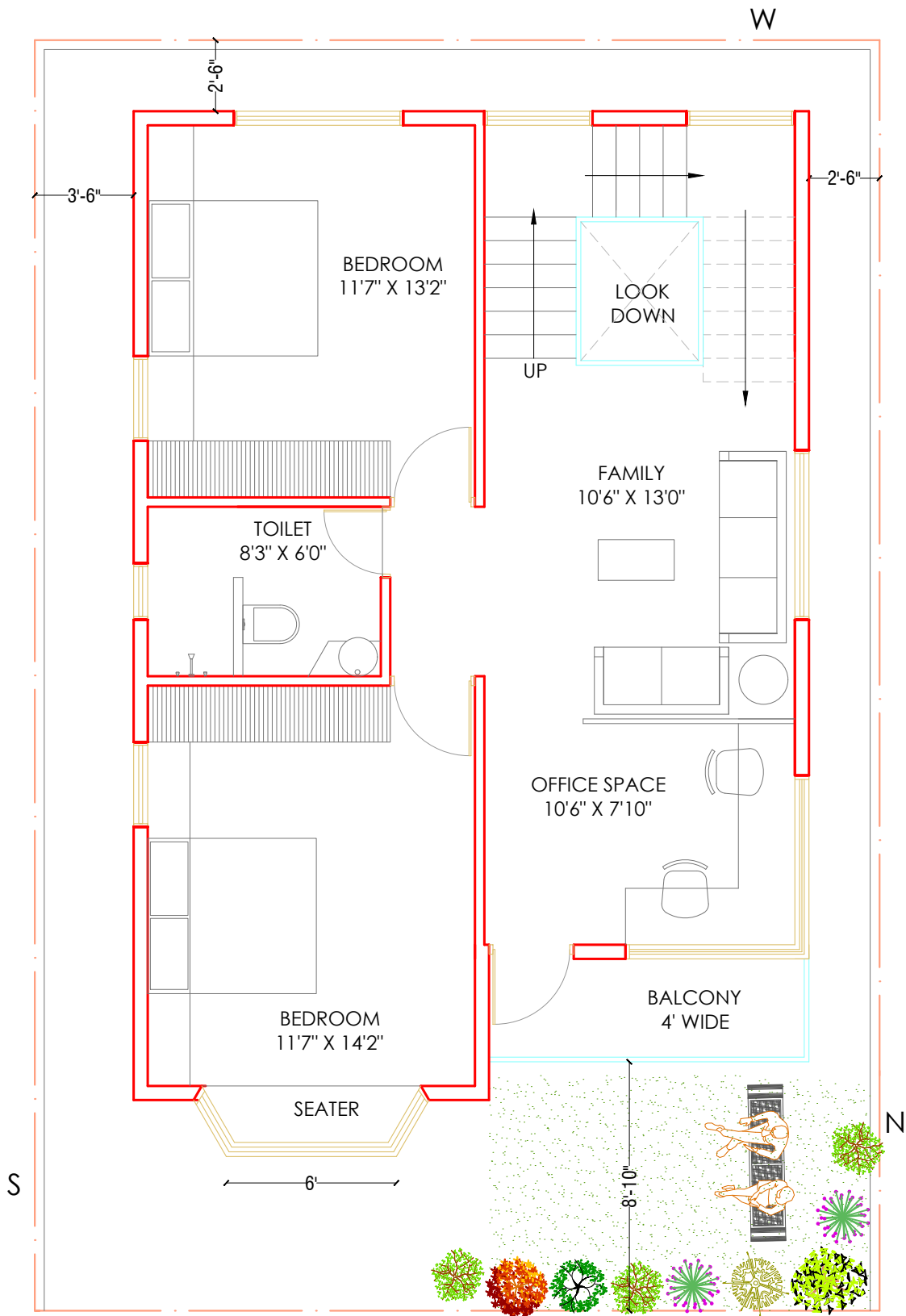
FIRST FLOOR PLAN BUILTUP AREA:- 795 SFT BALCONY :- 41 SFT
